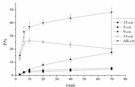
Figure 4. The trend of each Z-isomers and total amount with the processing time at 115°C
