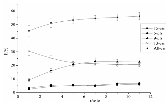
Figure 8. The trend of each Z-isomers and total amount with the processing time at 145°C
