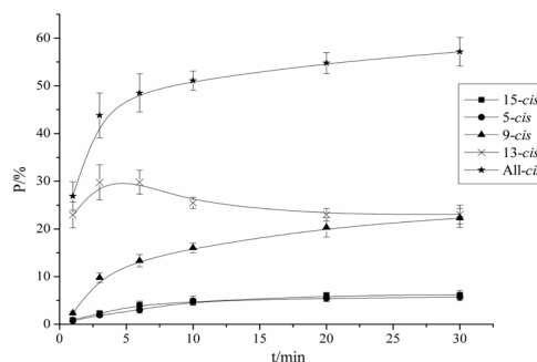
Figure 6. The trend of each Z-isomers and total amount with the processing time at 130°C
