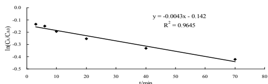
Figure 5. First order plot for the degradation of lycopene in simulation system during heating at 115°C
