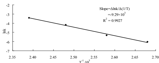
Figure 10. Plot of \ln(k) vs. (T^{-1}) for lycopene degradation during heating
