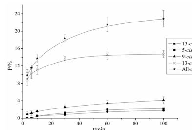
Figure 2. The trend of each Z isomers and total amount with the processing time at 100°C
