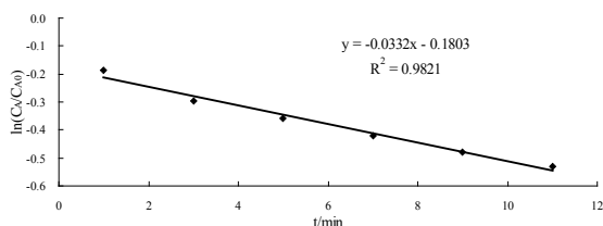
Figure 9. First order plot for the degradation of lycopene in simulation system during heating at 145°C
