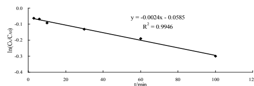
Figure 3. First order plot for the degradation of lycopene in simulation system during heating at 100°C
