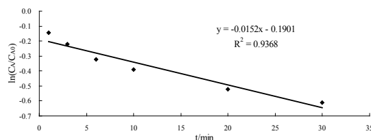
Figure 7. First order plot for the degradation of lycopene in simulation system during heating at 130°C
