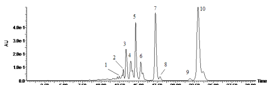
Figure 1. HPLC chromatogram of lycopene in simulation system after heating at 130°C for 10 min
